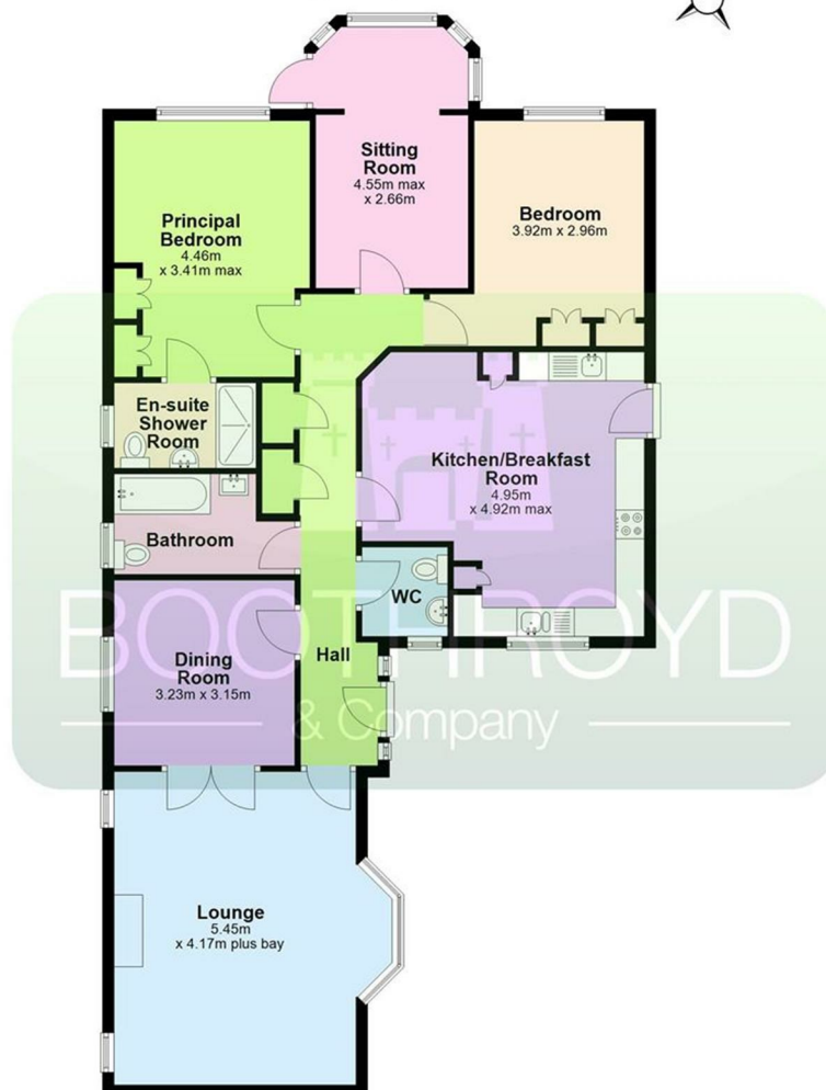
Ground Floor Approx. 120.8 sq. metres
